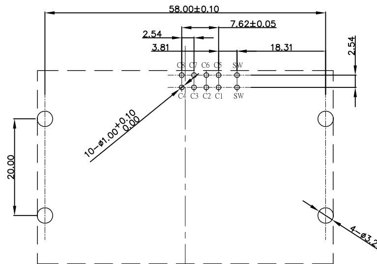
RECOMMENDED PCB LAYOUT TOL.:±0.05
