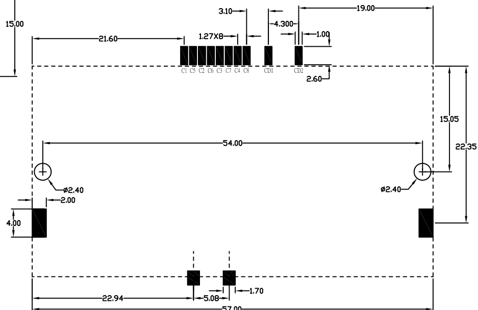
RECOMMENDED PCB LAYOUT TOL:±0.05
